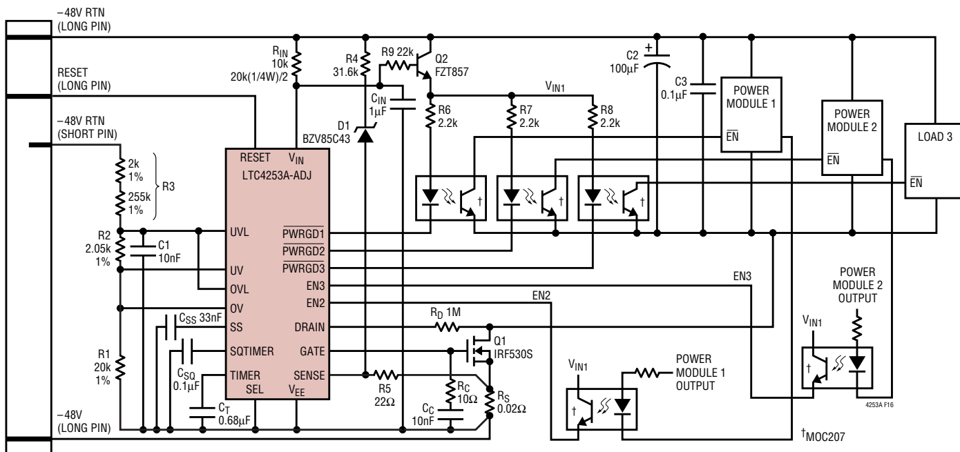
Figure 16. Power Limit Circuit Breaker Application
